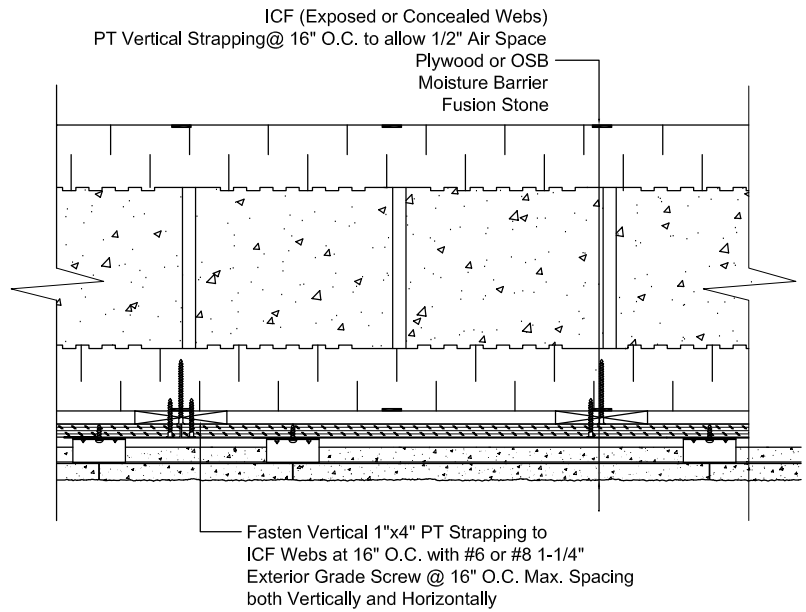
Typical Cross Section ICF Wall - Plan View
