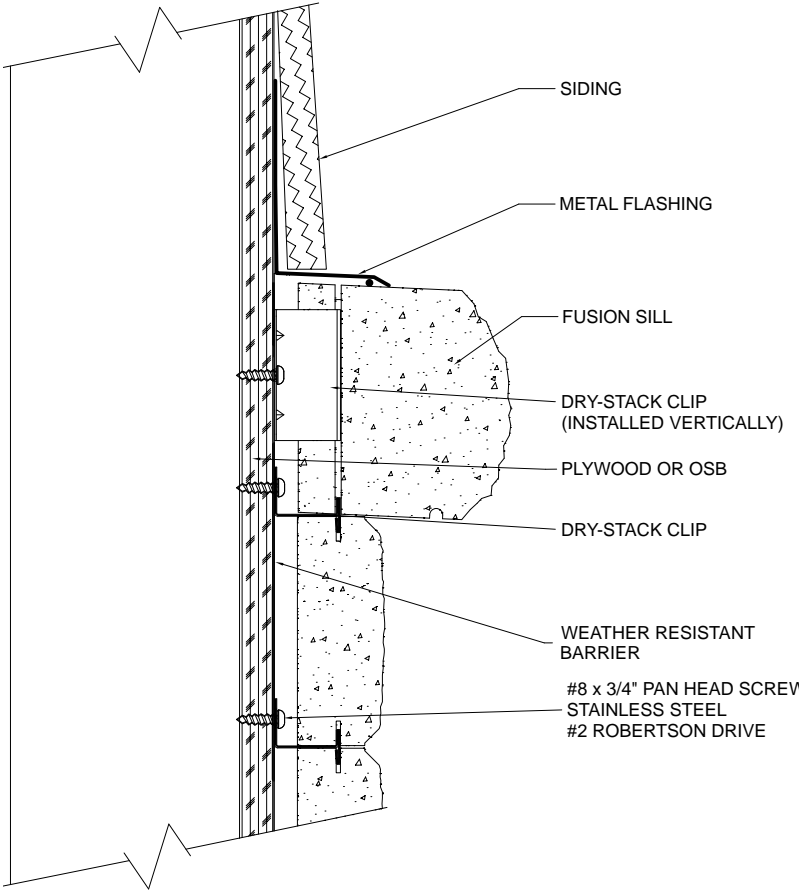
Typical Cross Section Wainscot Sill Transition to Siding
